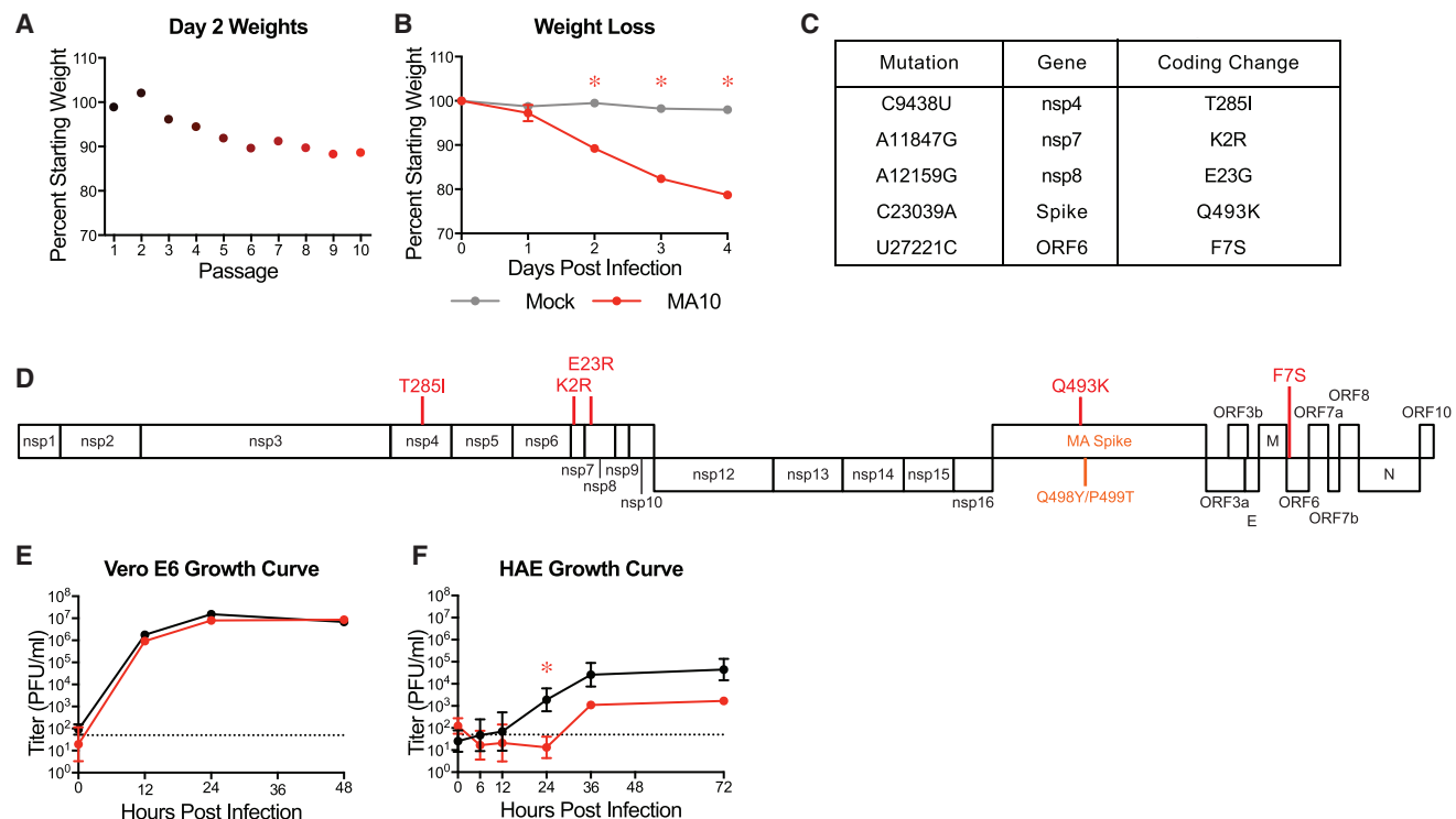
Figure 1. SARS-CoV-2 MA Increases in Pathogenicity following Serial In Vivo Passage in Mice
