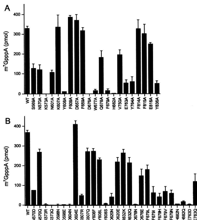
FIGURE 3. Mutational effects on vaccinia virus cap methyltransferase activity. The extents of 3 H-m 7 GpppA formation by wild-type and mutant D1-C/D12 heterodimers are plotted with alanine mutants surveyed in A and conservative mutants in B . Each datum is the average of three experiments; standard error bars are shown.
